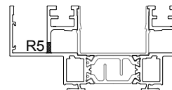
Corte | Cut | Coupe E-E
