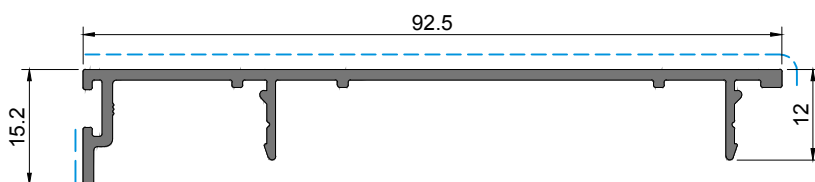
JT 88 Capa Cover | Capot
