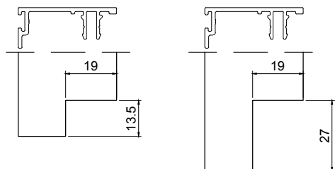
Perfis | Profiles | Profilés JT85 e | and | et JT 88
