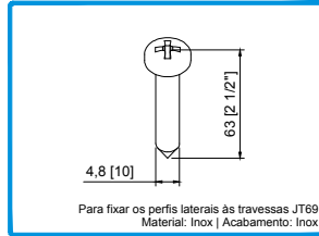
290087 PARAF. DIN7981 PH 4,8x63 INOX A2
