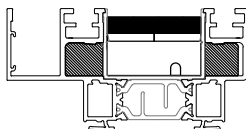
Corte | Cut | Coupe C-C
