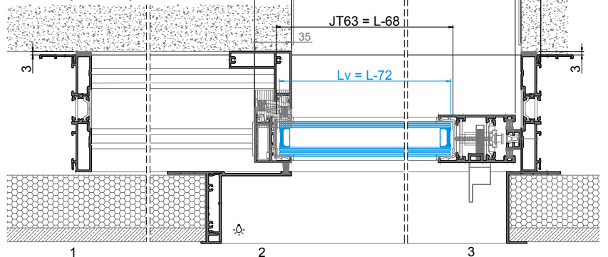
Fechado | Closed | Fermé
