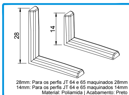
210239 TOPO JT64/JT65 28MM 210240 TOPO JT64/JT65 14MM
