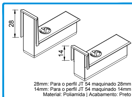
210243 TOPO CENTRAL REFORÇ. JT54 28MM
