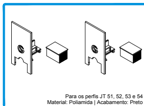
212339 CONJ. TAMPAS TOPOS CENTRAIS JT
