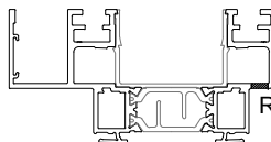
Corte | Cut | Coupe B-B
