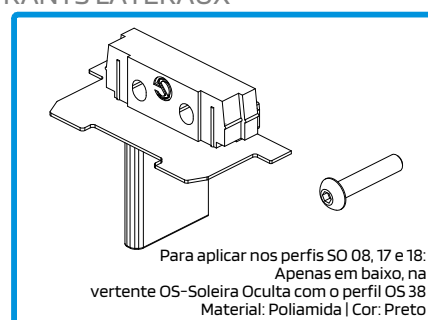
210191 TOPO LATERAL INF. 40mm N°20 OS-V3 SOL. INVIS.
