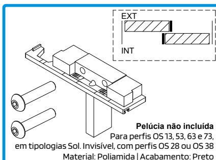
210985 TOPO CENTRAL Nº15 OS-T SOL. OCULTA DIR
