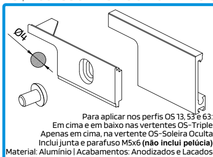
212434 CONJ. TOPO CENTRAL Nº12 OS-T DRT
