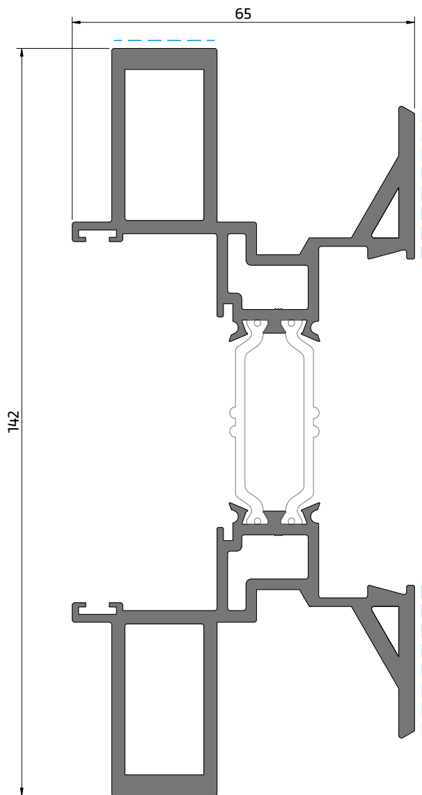
OS 88 Perfil união 3/4 folhas 3/4 Leaves connecting profile Profilé pour connexion 3/4 ventaux
