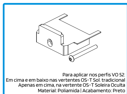
210304 TOPO LATERAL SUP. INF. N°24 OS-T FECH.
