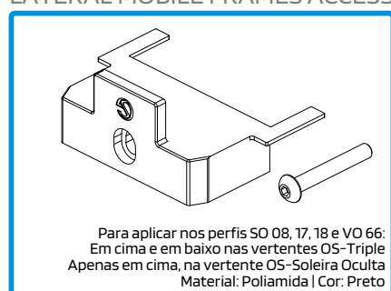
210189 TOPO LATERAL SUP. INF. N°18 OS-V3
