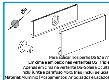
212435 CONJ. TOPO CENTRAL INVERT Nº13 OS-T
