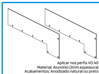
212210 CONJ. TOPOS CALEIRA/SOLEIRA OS-T 2-RAIL
