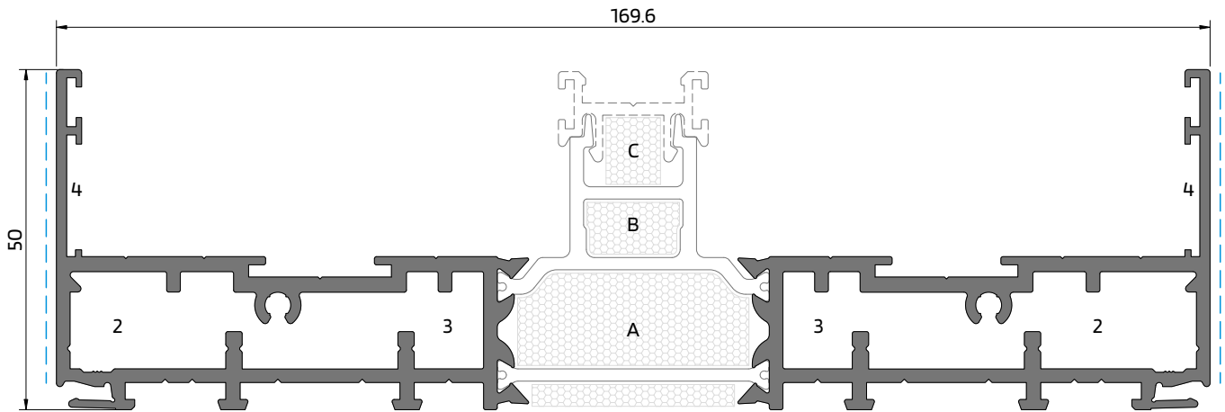
VO 41 Ombreira/padieira 2-rail 2-rail Jamb/lintel | Jambage/linteau 2-rail
