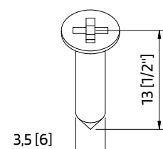
290050 PARAF. DIN7982 PH 3,5x13 INOX A2
