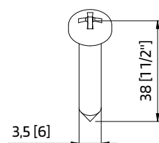
290082 PARAF. DIN7981 PH 3,5x38 INOX A2
