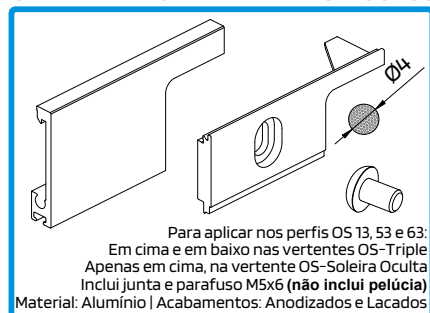
212433 CONJ. TOPO CENTRAL Nº12 OS-T ESQ
