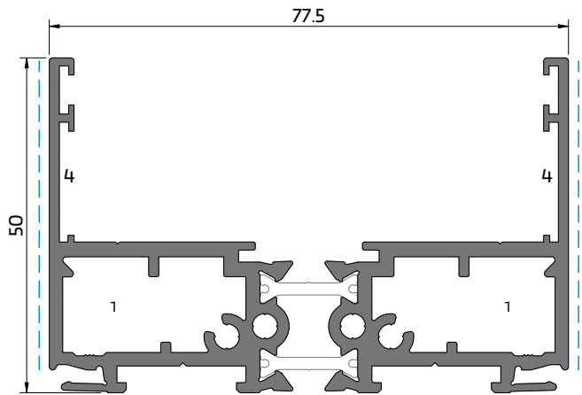
SO 44 Ombreira/padieira 1-rail 1-rail Door jamb/Intel | Jambage/linteau 1-rail
