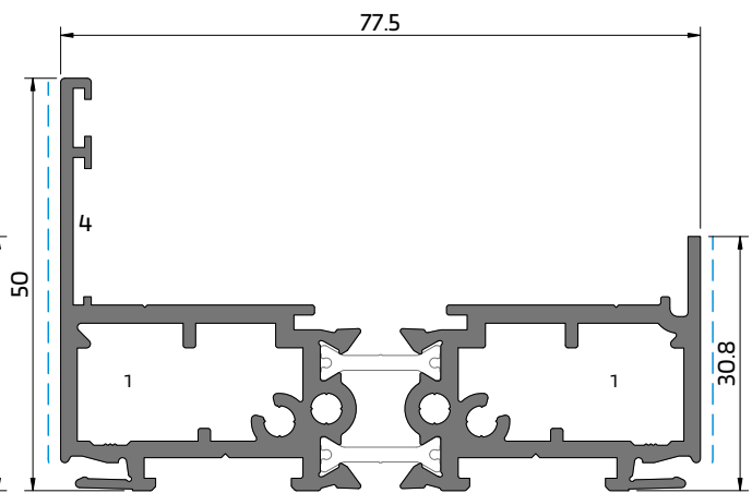
SO 55 Ombreira/padieira 1-rail 1-rail Door jamb/Intel | Jambage/linteau 1-rail
