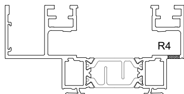
Rasgo | Hole | Rainure R4: 6x35mm
