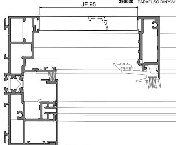
290030 PARAFUSO DIN7981 4,2x38 INOX A2
